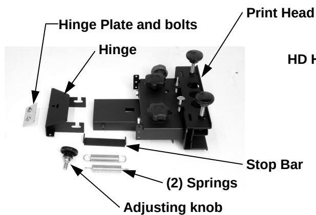
Standard Print Head
