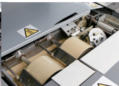
Glue drums with automatic side gluing and glue cut off control
